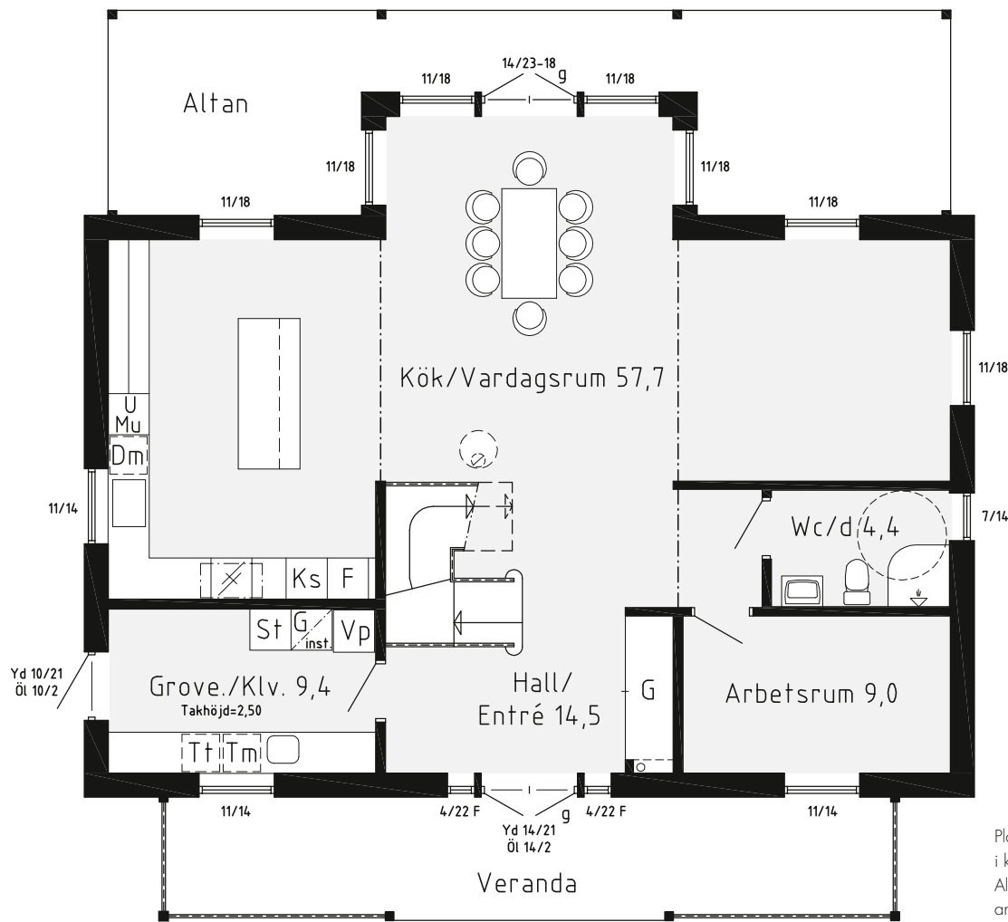
BOTTENPLAN
