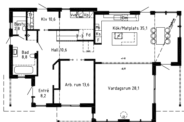
BOTTENPLAN
