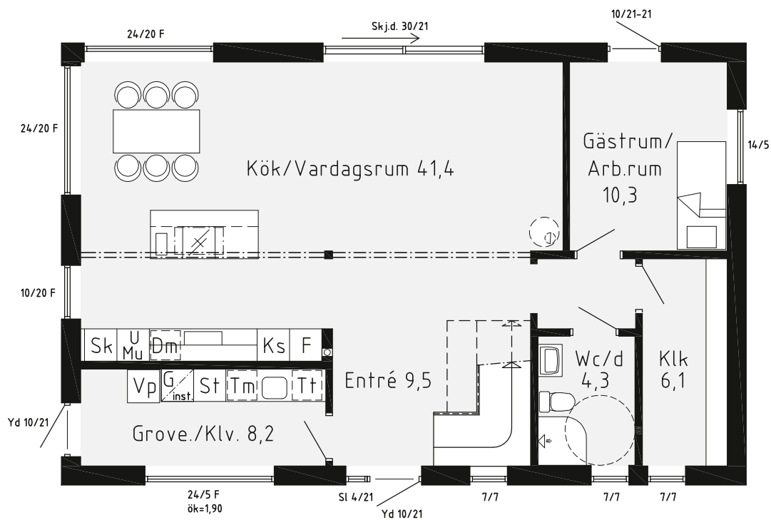
BOTTENPLAN
