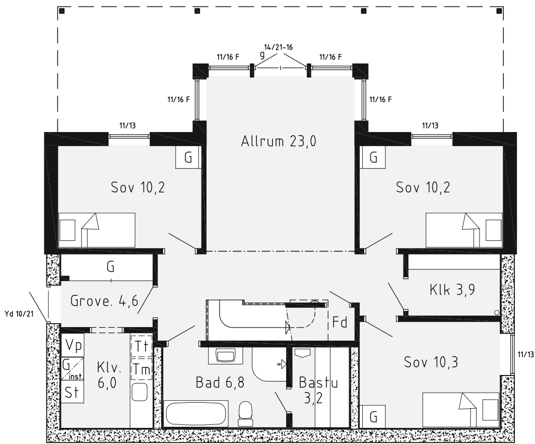
BOTTENPLAN
